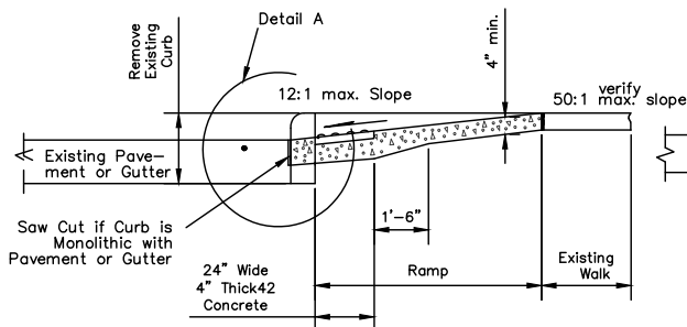
SECTION A-A EXISTING WALK DETAIL
