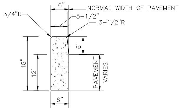
BARRIER CURB
