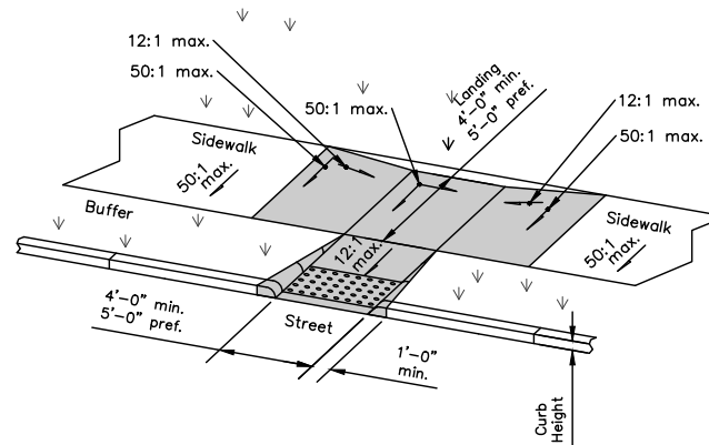
Type C2 (Combined with returned curb)
