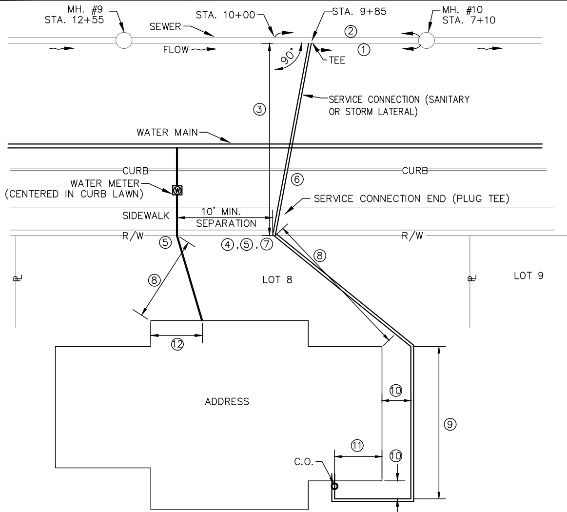
SAMPLE SITE SKETCH
