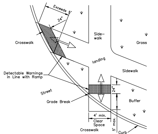
DETECTABLE WARNING ALIGNMENT
