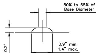
HEIGHT AND DIAMETER
