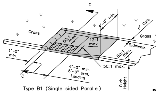
Type B1 (Single sided Parallel)
