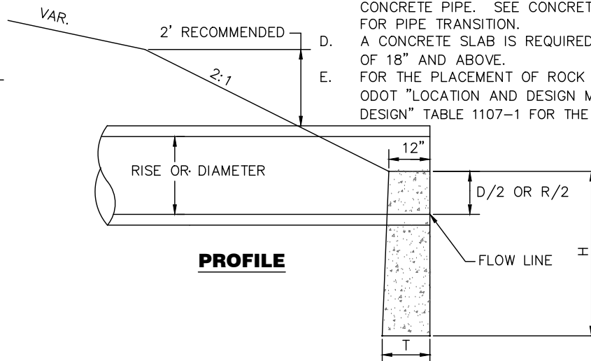
HEADWALL FOR CONCRETE PIPE
