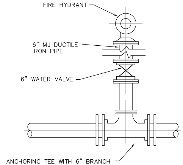
BASIC TEE DETAIL PLAN
